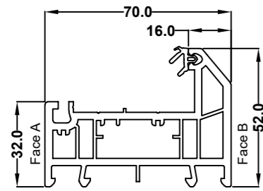
52mm Outer Frame 70C 546815 White 586815 Foiled
