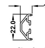
Chamfered Astragal Bar 559251 White 589251 Foiled
