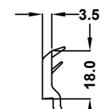
36mm Flush Sash Square Bead 637533 White only
