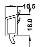
36mm Flat Bead 560590 White 596910 Foiled
