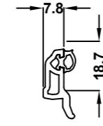
44mm Ovlo Bead 546860 White 586865 Foiled
