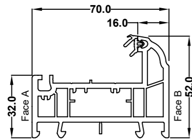
52mm Outer Frame 70S 546415 White 586415 Foiled
