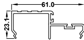
Aluminium Tread Plate 318011
