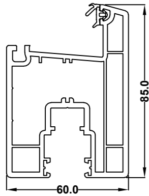
Door Sash 500563 White 585453 Foiled
