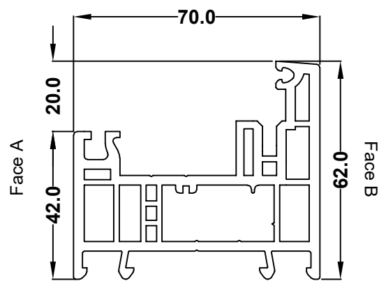
62mm Outer Frame White 546930 Foil 586930
