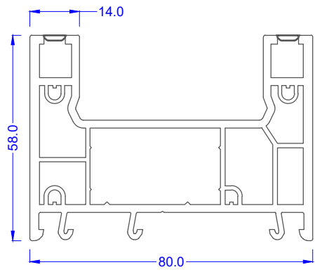
Outer Frame 575602 White 595802 Foiled
