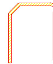
34.5 x 40.8 x 2mm Reinforcement 357832 361488 Pre-routed
